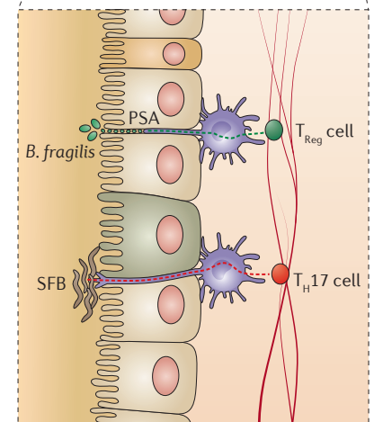
Figure 2 | Microbiota-induced maturation of the gastrointestinal tract. The microbiota promotes substantial changes in gut morphology, including villus architecture, crypt depth, stem cell proliferation, blood vessel density, mucus layer properties and maturation of mucosa-associated lymphoid tissues. a | In germ-free mice, the villi in the distal small intestine are longer and thinner and have a less complex vascular network than the villi of conventionally raised animals. In the absence of bacteria, intestinal crypts are less deep and contain fewer proliferating stem cells. Furthermore, germ-free animals show reduced mucus thickness and altered mucus properties. b | Moreover, very few isolated lymphoid follicles, immature Peyer's patches and immature mesenteric lymph nodes (MLNs) are present under germ-free conditions, and levels of both immunoglobulin A (IgA) and antimicrobial peptides (AMPs) are lower than in conventionally raised animals. c | In conventionally raised mice, polysaccharide A (PSA) of Bacteroides fragilis is known to induce the expansion of CD4 + CD25 + FOXP3 + regulatory T (T Reg ) cells, which have an anti-inflammatory effect and dampen immune responses. By contrast, segmented filamentous bacteria (SFB) have been shown to induce the expansion of T helper 17 (T H 17) cells, which are pro-inflammatory.
